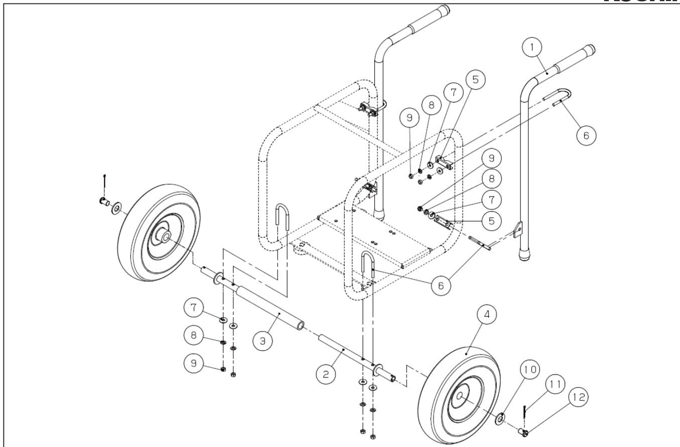
DWG No.013856601 MODEL : WK-12A FORM : WK-12A-BAA-0
