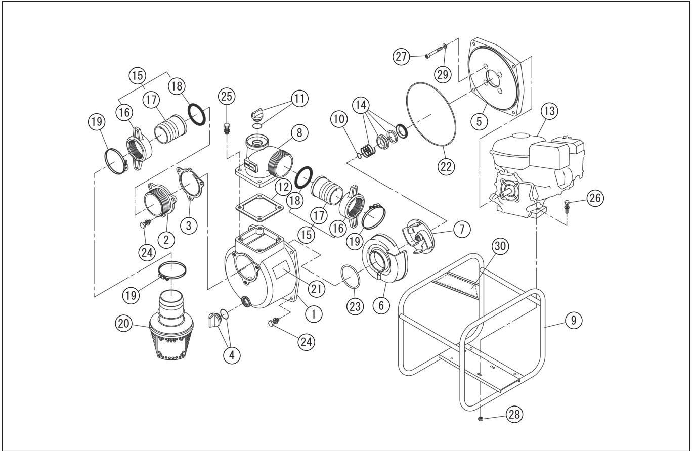
DWG No.012933010 MODEL : SEV-80X FORM : SEV-80X-BAU-2 (K180)
