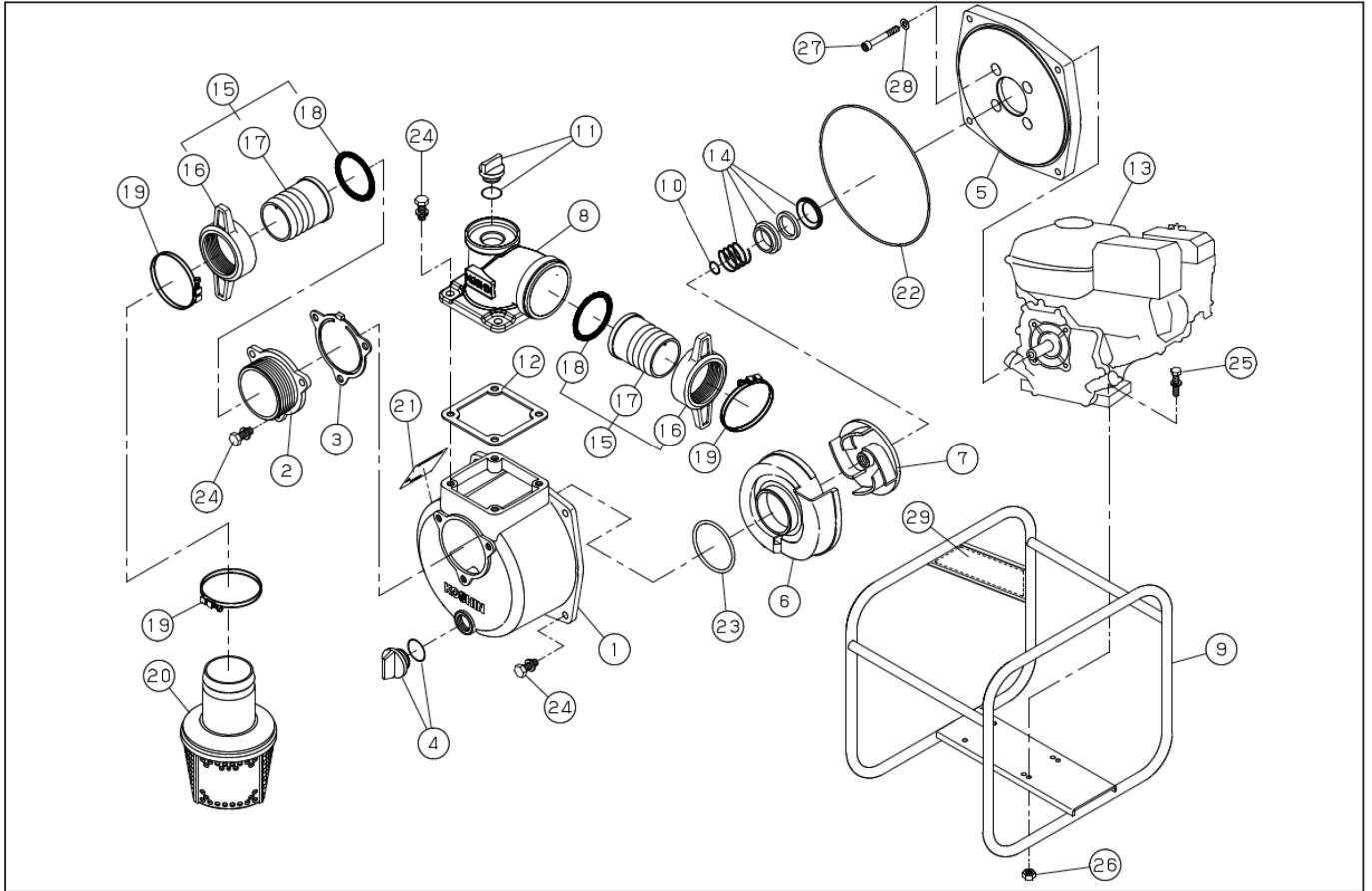
DWG No.012932612 MODEL : SEV-80X FORM SEV-80X-BAT-2
