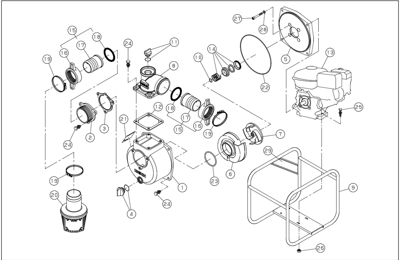
DWG No.012923412 MODEL : SEV-80X FORM SEV-80X-BAN-3
