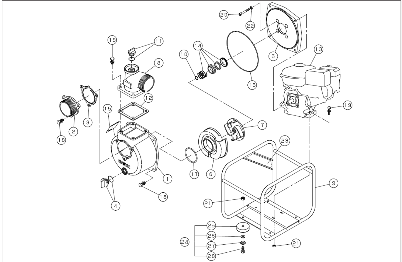
DWG No.013857901 MODEL : SEV-80E FORM : SEV-80E-BAC-0 (K210S)
