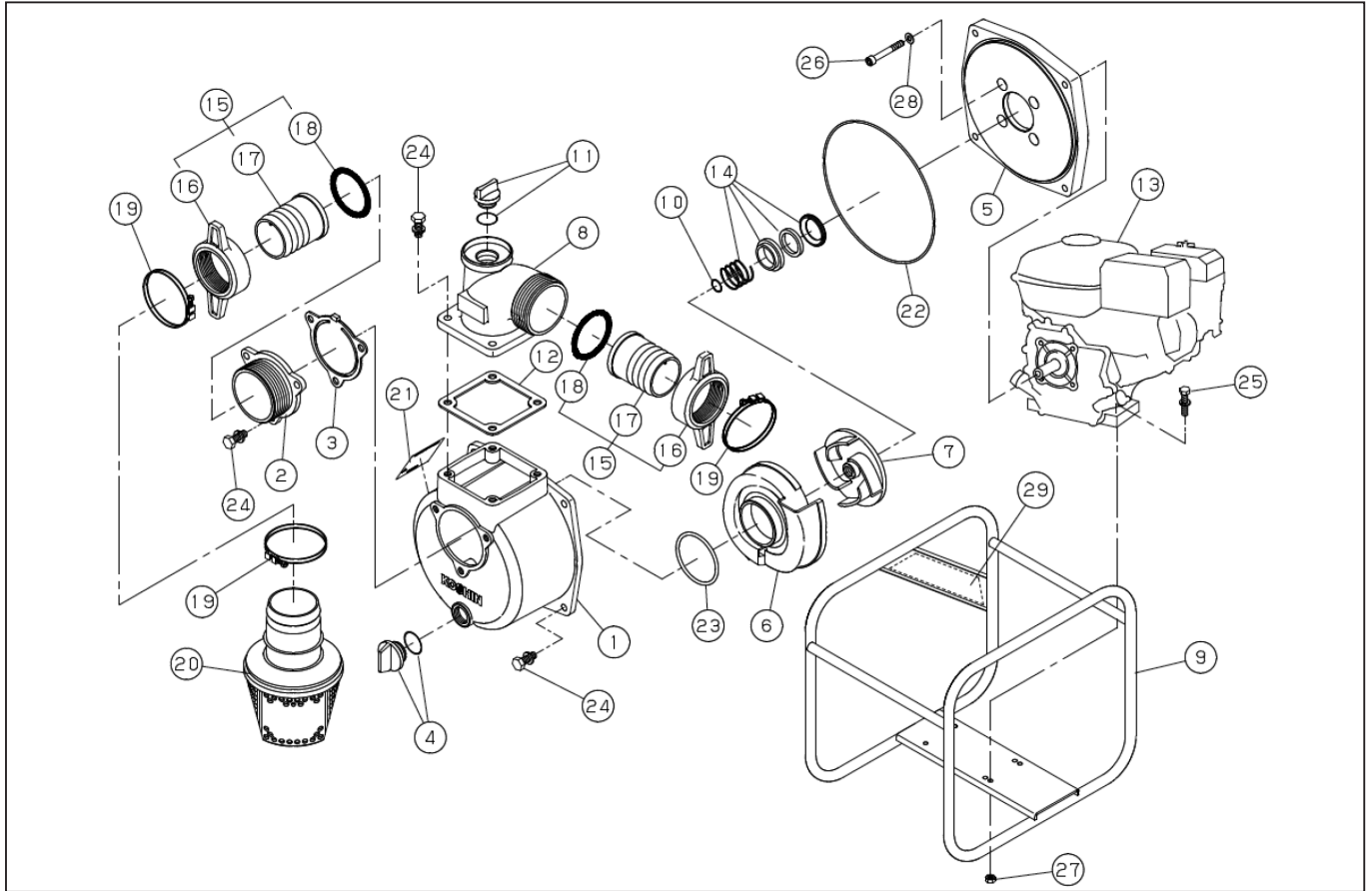
DWG No.013857501 MODEL : SEV-80E FORM : SEV-80E-BAB-0 (K210S)
