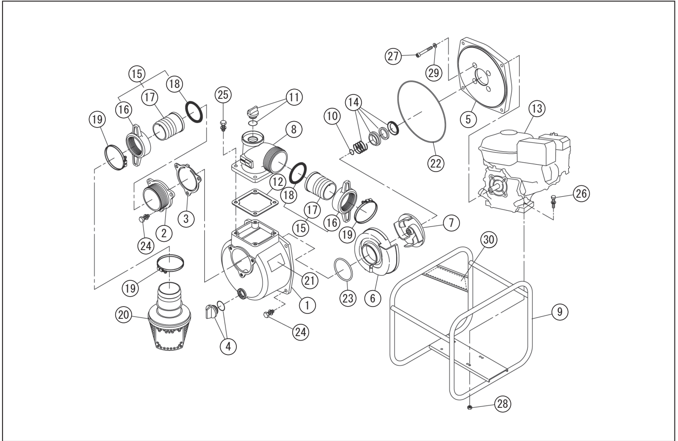
DWG No.012933901 MODEL : SEH-80X FORM : SEH-80X-BFP-0 (GX160H1)
