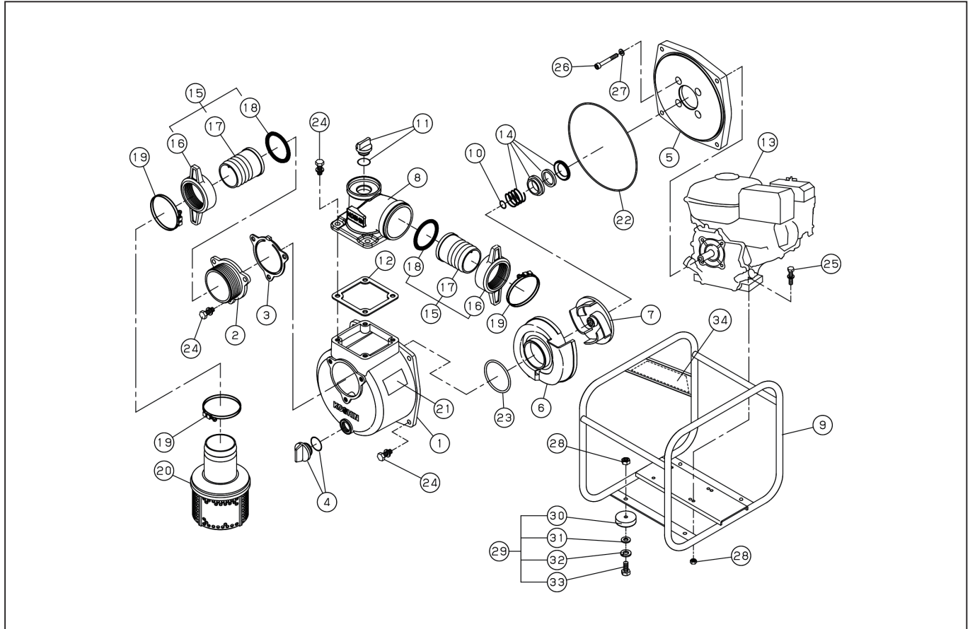
DWG No.012924213 MODEL : SEH-80X FORM : SEH-80X-BFH-2(GX160H2)
