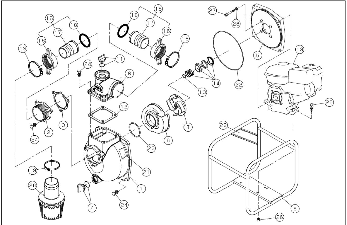
DWG No.012928209 MODEL : SEH-80JP FORM : SEH-80JP-BAA-1 (GP160)
