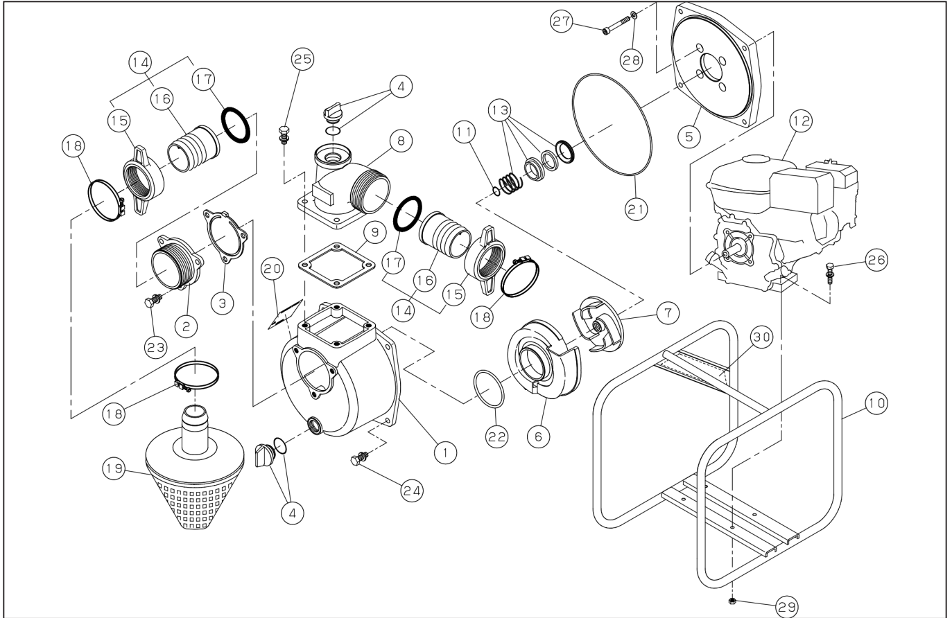
DWG No.013864201 MODEL : SEH-50X FORM : SEH-50X-BGN-0 (GX120WBT)
