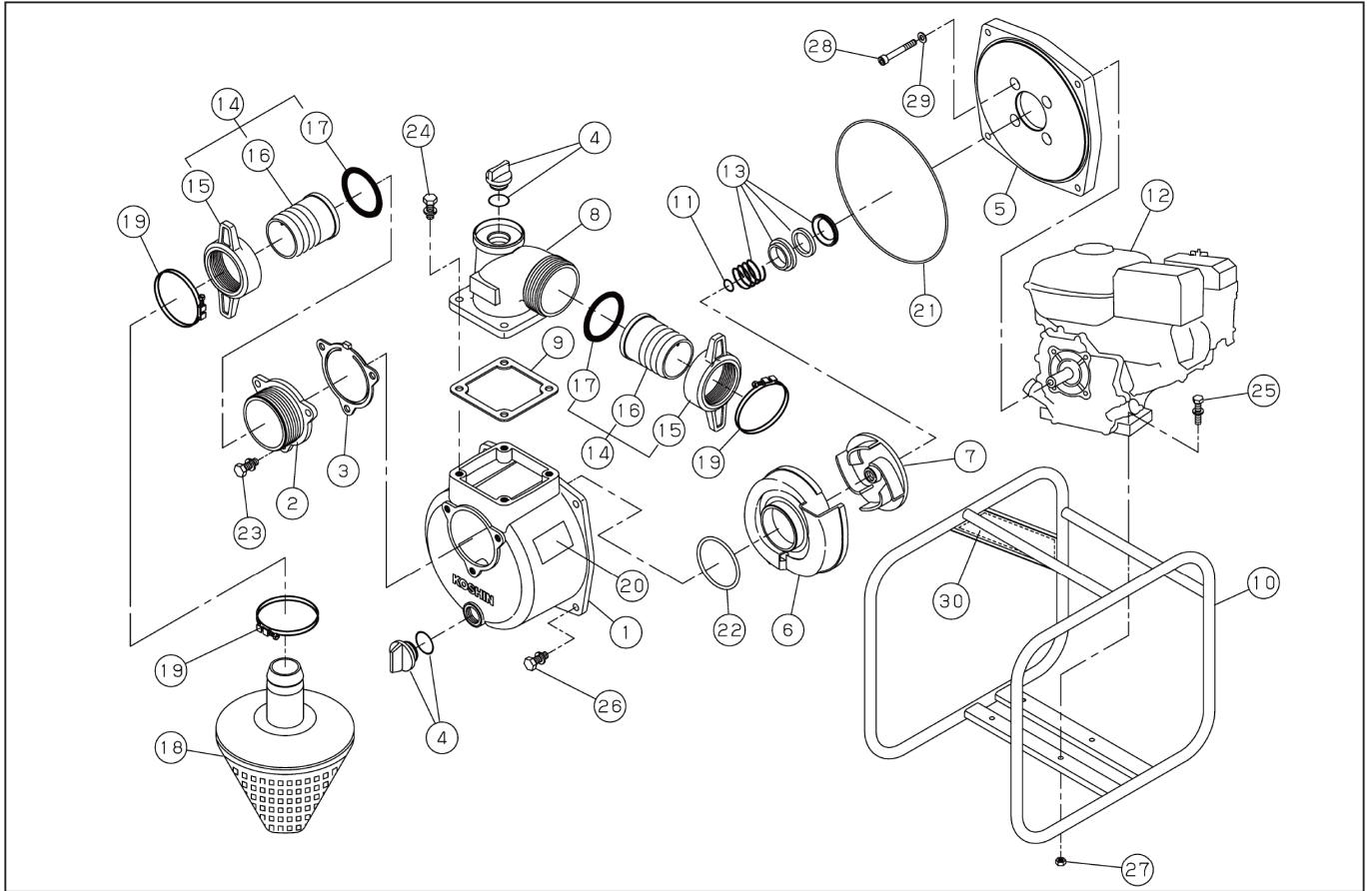
DWG No.013863501 MODEL : SEH-50X FORM : SEH-50X-BGK-0 (GX160UH2)
